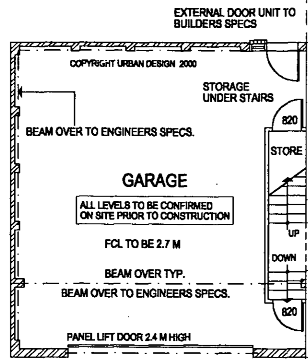
LOWER FLOOR PLAN GARAGE AREA - 65.84 SQM / 7.08 SQ INCLUDING STAIRS
