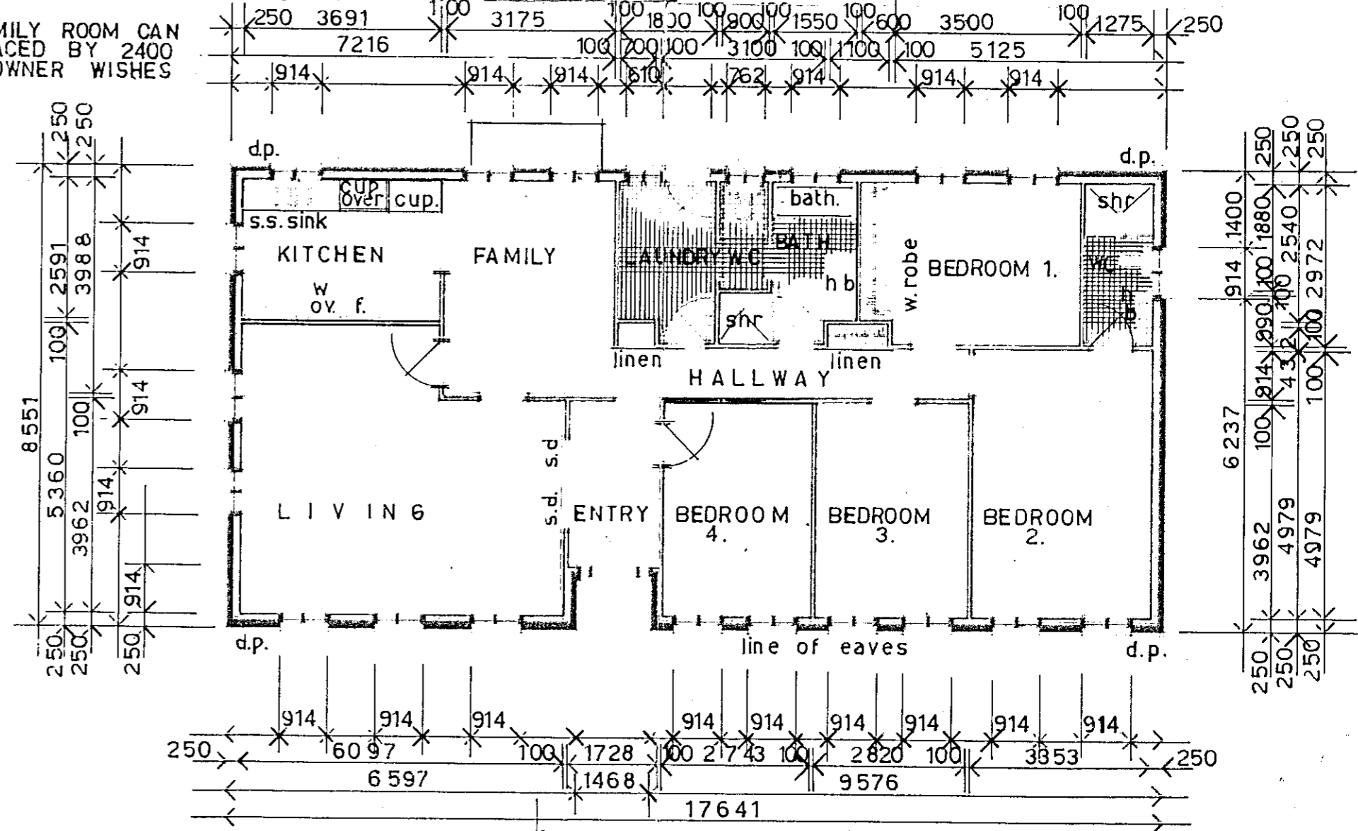
FLOOR PLAN
