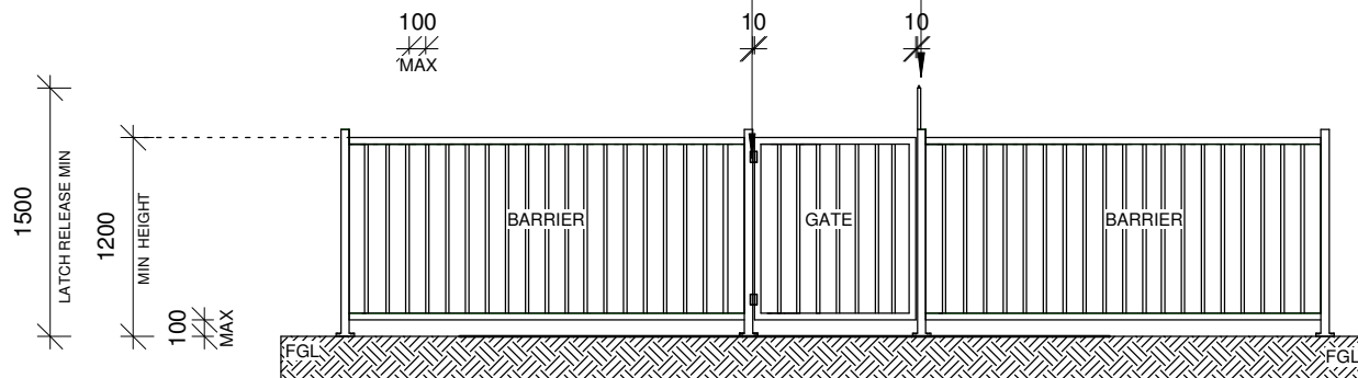
FRONT ELEVATION TYPICAL ALUMINIUM POOL BARRIER
