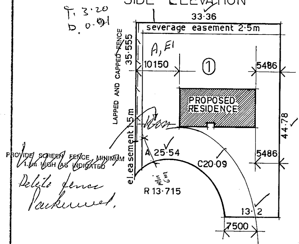
SITE PLAN
