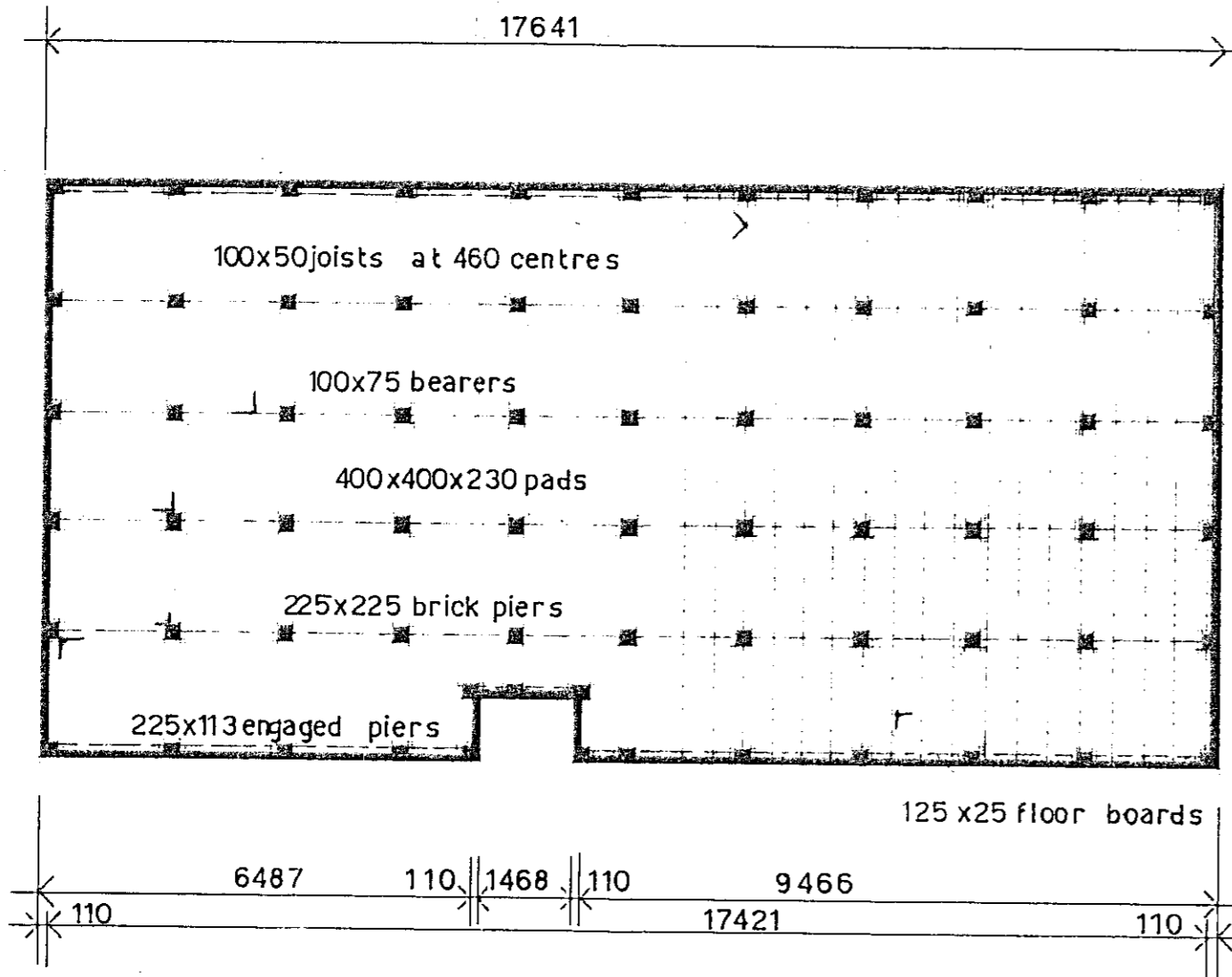
FOUNDATION PLAN
