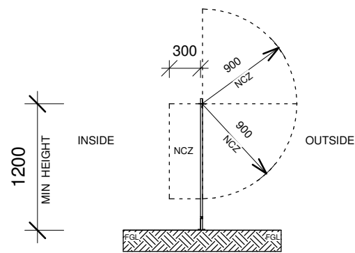
SIDE ELEVATION TYPICAL METAL POOL BARRIER
