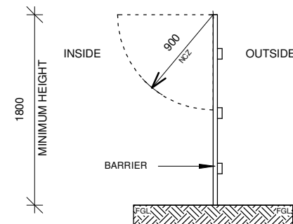
SIDE ELEVATION TYPICAL BOUNDARY BARRIER
