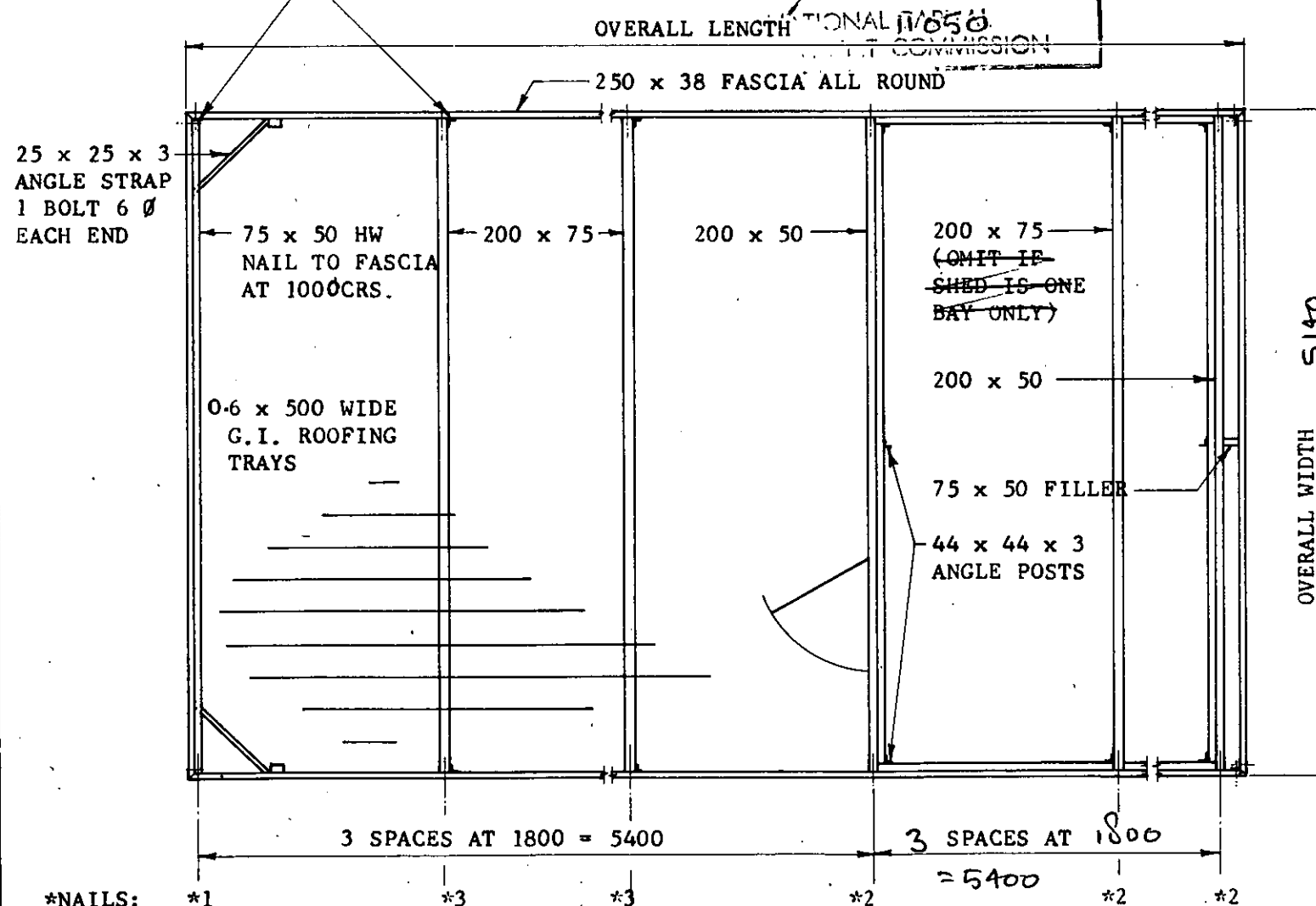
PLAN (NOT TO SCALE)
