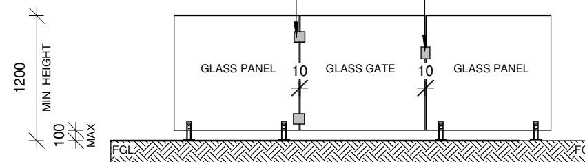
FRONT ELEVATION TYPICAL GLASS POOL BARRIER
