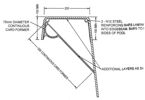
EDGE BEAM DETAIL SCALE 1:5
