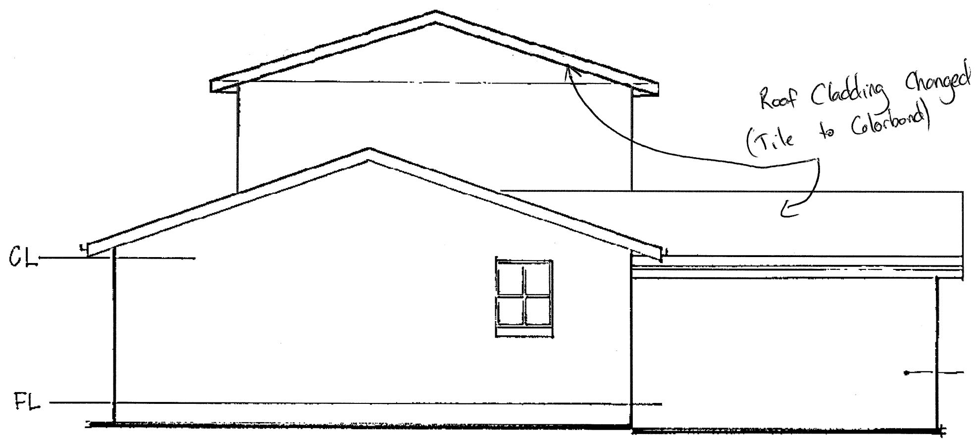
SIDE ELEVATION C
