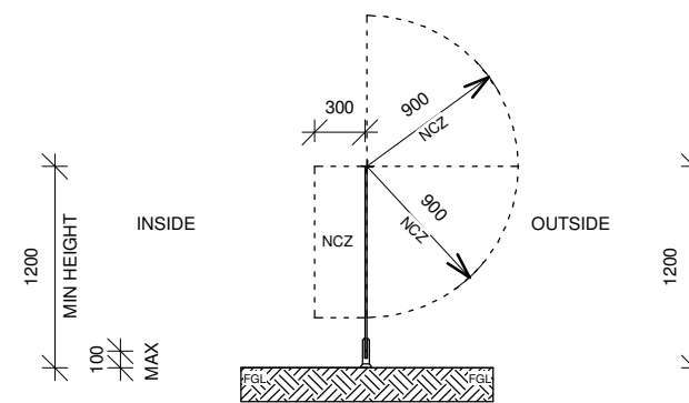
SIDE ELEVATION TYPICAL GLASS POOL BARRIER
