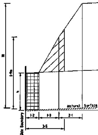
Natural surface rising from side boundary
