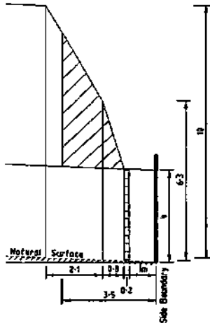
Natural surface rising from side boundary
