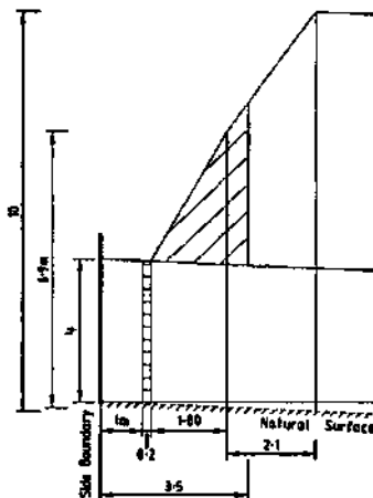
Natural surface falling from side boundary
