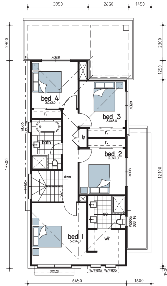
FIRST FLOOR 1:100
