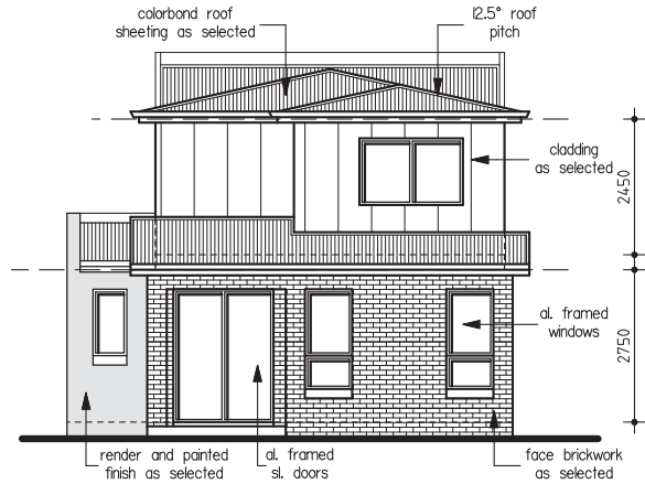
REAR FACADE 1:100
