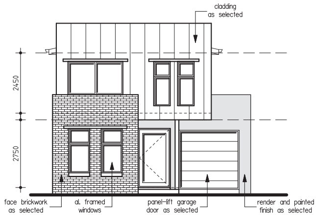
FRONT FACADE 1:100
