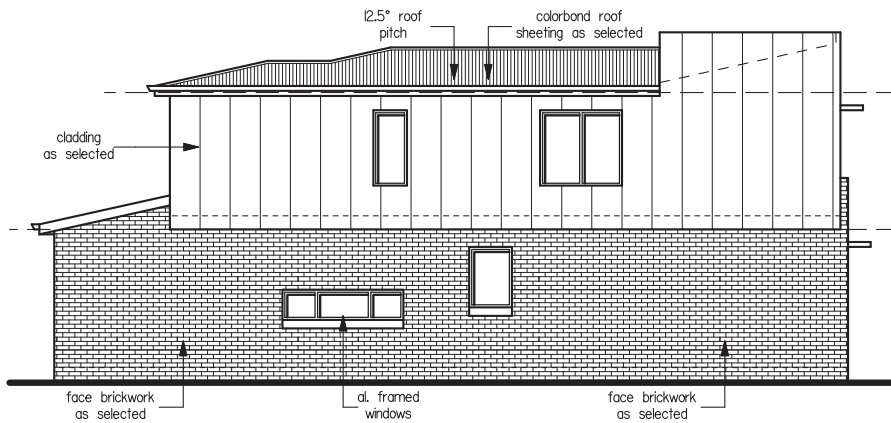
SIDE FACADE 1:100
