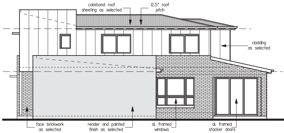
SIDE FACADE 1:100
