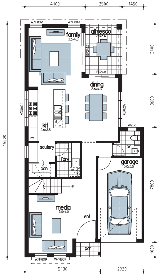
GROUND FLOOR 1:100
