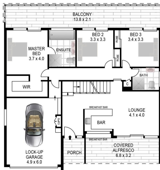
ENTRY FLOOR
